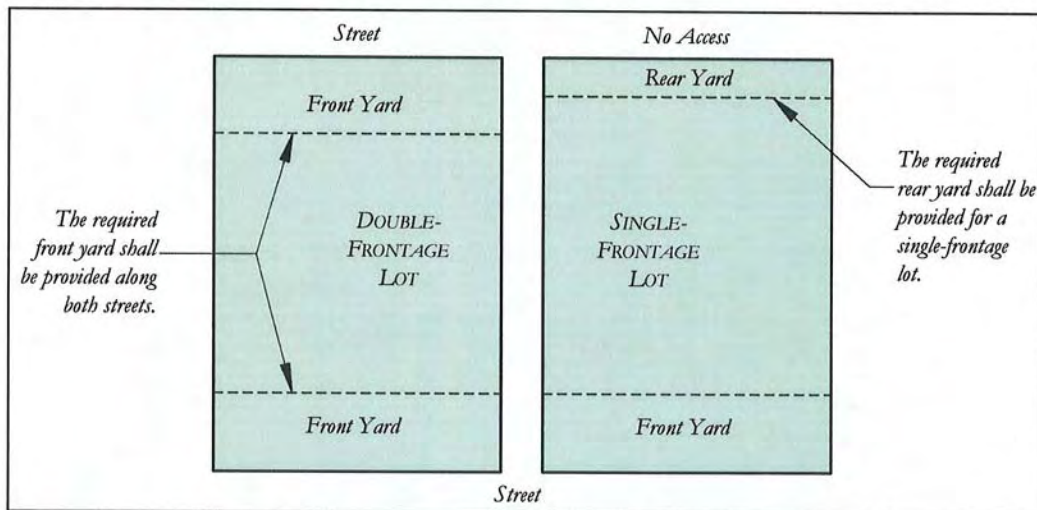
Illustration 43-3: Double-Frontage Lots
