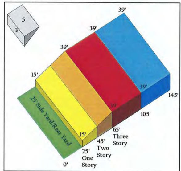
Illustration 22-2: Setback & Height Relationship for Multiple-Family Structures
