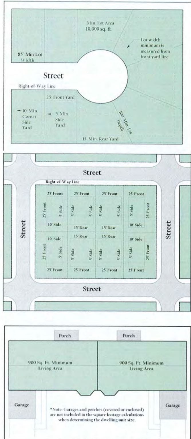
Illustration 20-2: Lot, Yard & Floor Area Regulations for the Duplex District
