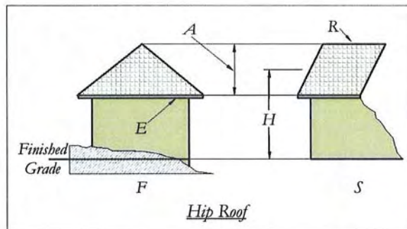
Illustration 45-1: Measuring Building Height
