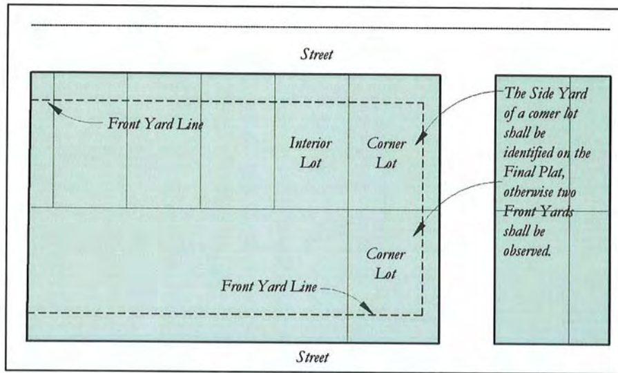
Illustration 43-2: Corner Lots
