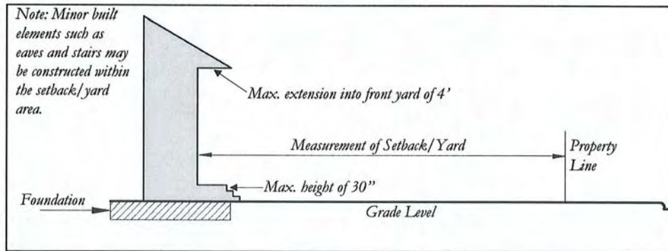
Illustration 43.4: Measuring Front Yard
