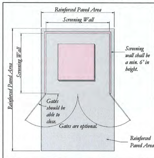
Illustration 42-1: Refuse Area Screening
