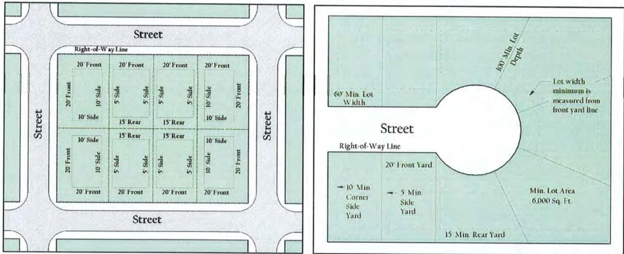
Illustration 17-1: Lot & Yard Regulations for the SF-6 District
